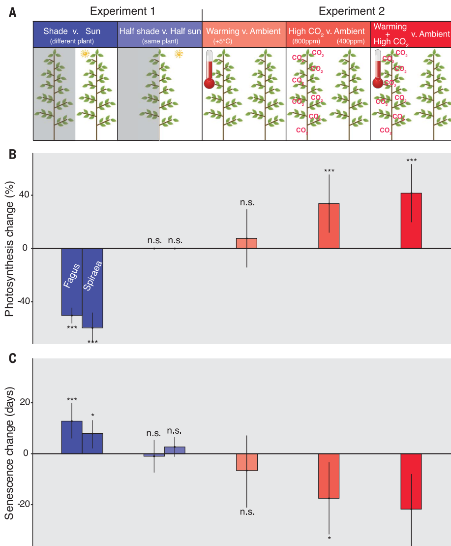
Fig. 2. Experimental tests of the effects of plant-level photosynthesis on autumn senescence dates. (A) Experimental setup.
